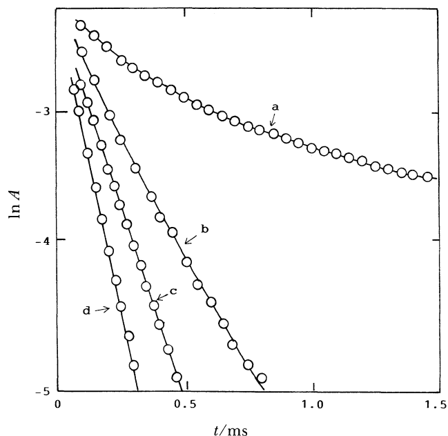
Fig. 2. First-order plots for decay of \text{Ph}_3\text{Sn}\cdot (at 330 nm) in the presence of t\text{-BuCl} in degassed cyclohexane; (a) 0, (b) 0.21, (c) 0.47, and (d) 0.70 \text{ mol dm}^{-3} .
